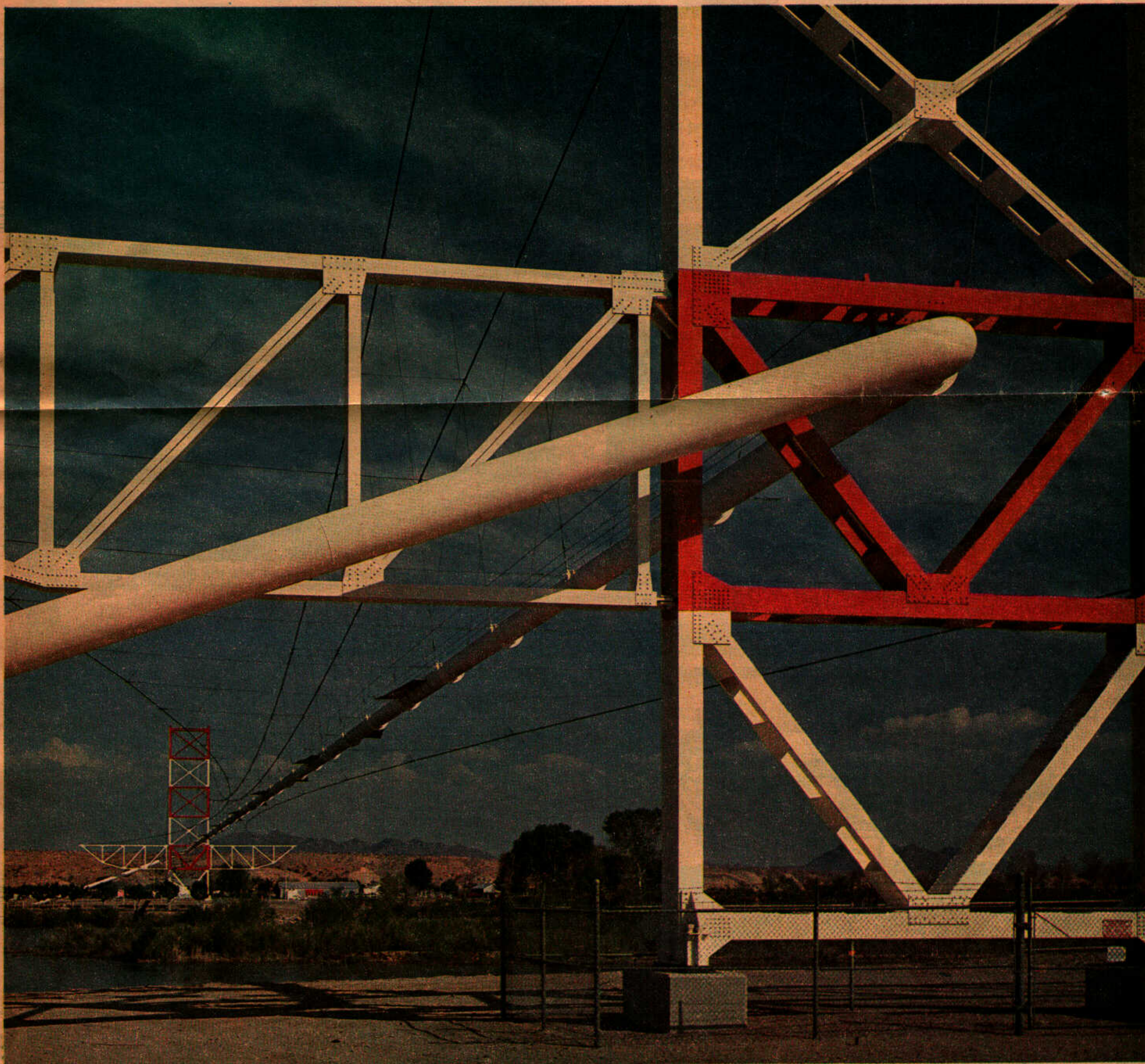
This pipeline bridge brings gas across the Colorado River near Blythe, California. Gas service by El Paso Natural to California began at this point in 1947. Since deliveries began, El Paso has had the lowest rates to California of any out-of-state supplier.
