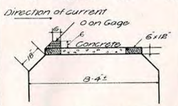
Cross Section of Dam Crest
