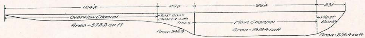
Average Cross Section for Stations 6, 8, 10, 12, 14, 16, 18 & 20
